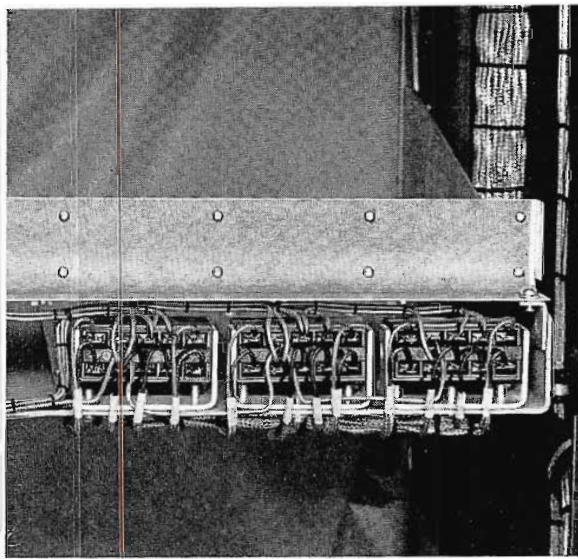
FIG. 3. Typical plug-in shelf wiring. Cover will be turned down to protect wiring after circuits are checked.
