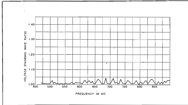
FIG. 8. Typical measured UHF standing wave ratio for RCA MI-19089-1 UHF transmission line.
