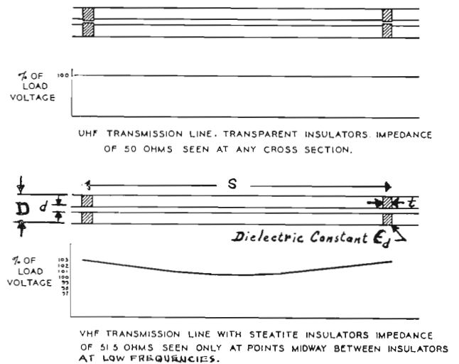
FIG. 6. Voltage distribution on UHF and VHF transmission lines.
