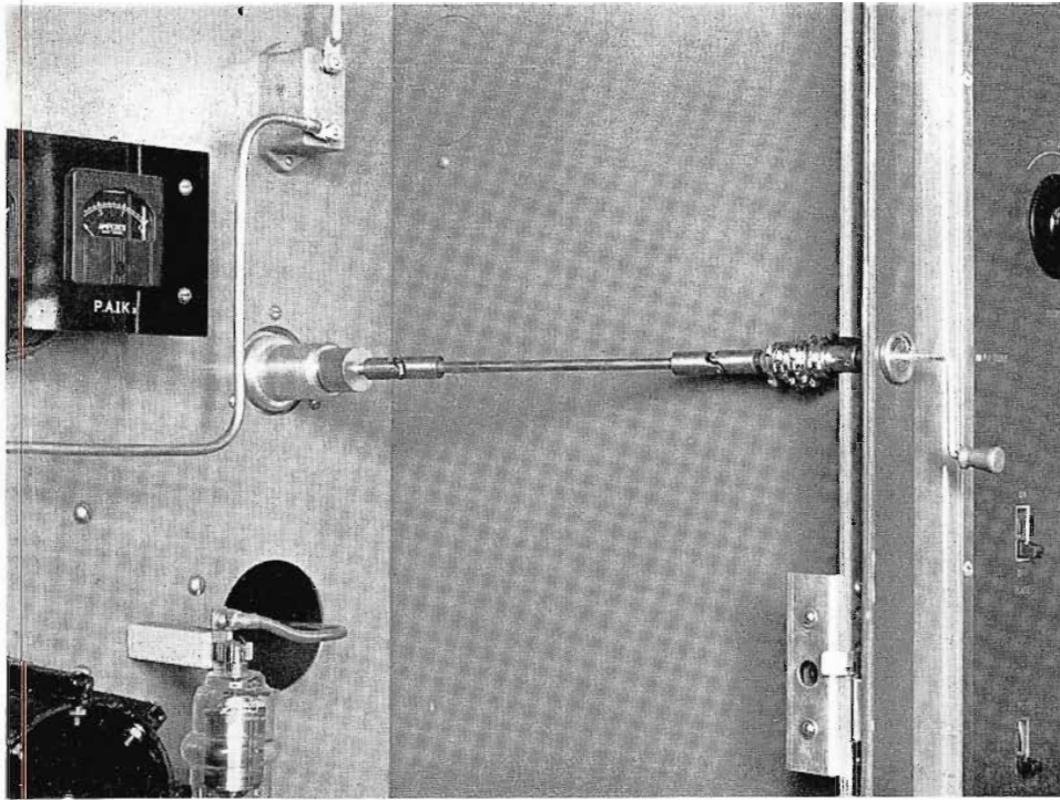
FIG. 16. View of mechanical power amplifier tuning control located on central control panel. Note door interlock switch at lower right.
