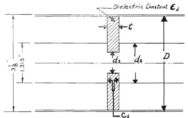
FIG. 7. Cross section of undercut insulator.
