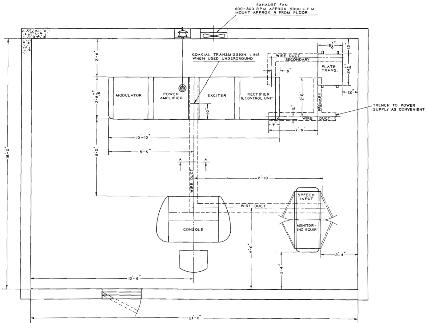
FIG. 21. Suggested floor plan arrangement of 5-kw AM Transmitter for a typical broadcast station.
