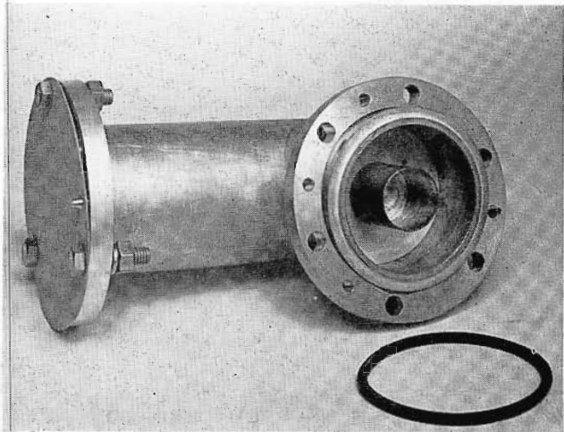
FIG. 10. MI-19089-2 UHF mitered elbow.
