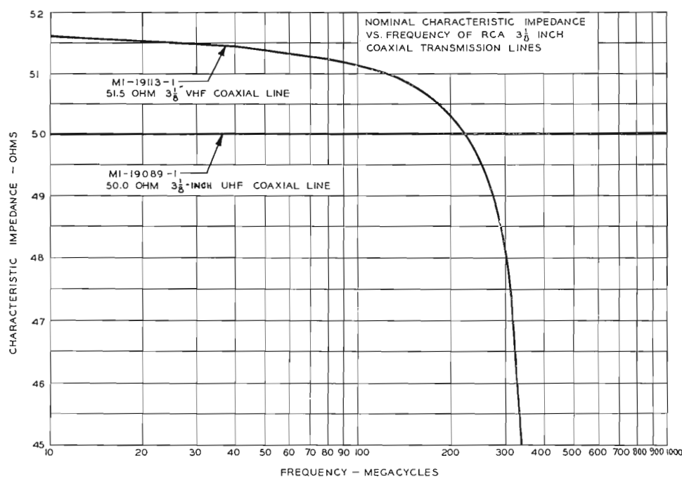
FIG. 2. Characteristic impedance of RCA 3 1/8" diameter coaxial lines.
