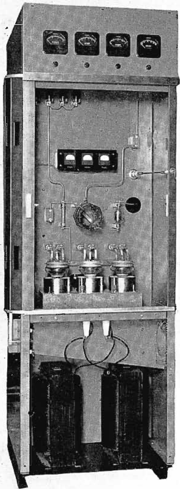
FIG. 18. Front view of power amplifier unit showing 5762 tubes.
