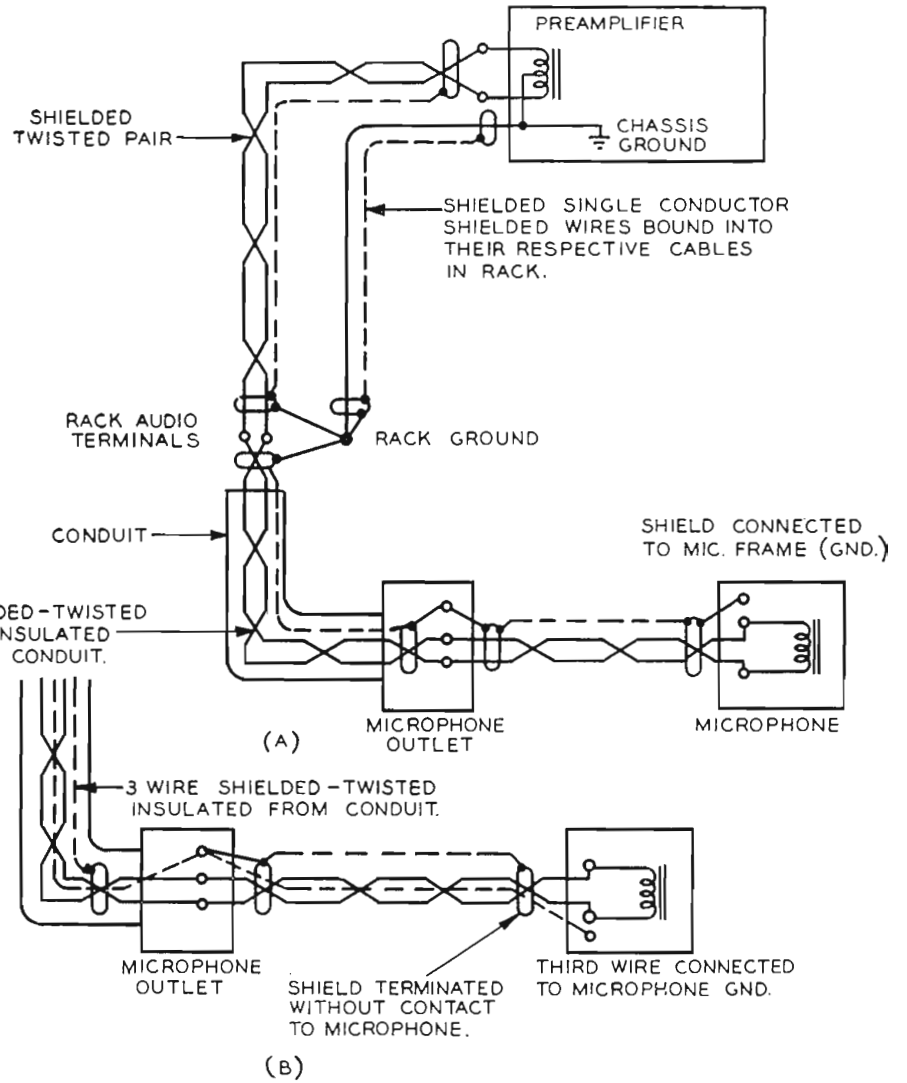
FIG. 4. Sketch showing typical microphone grounding practices.
