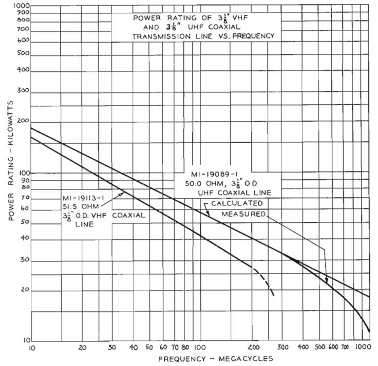
FIG. 4. Power rating of RCA 3/8" VHF and UHF coaxial lines.
