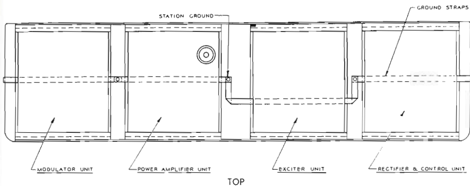
FIG. 2. Lower shows arrangement of cabinets and necessary connections for assembly. Upper shows base diagram of individual units.
