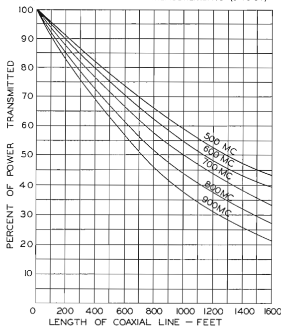
FIG. 9. Efficiency of RCA MI-19089-1 UHF coaxial line. TYPICAL 3 1/8 INCH O.D. UHF TRANSMISSION LINE EFFICIENCY BASED ON RCA MEASUREMENTS (5-16-51)
