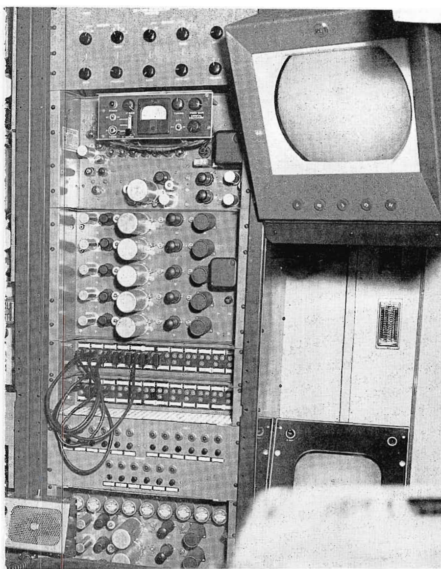
ARRAY of rack-mounted units surrounding the control desk in the receiving unit. From top to bottom in the left-hand rack are two heavy duty power supplies, the two-way radio communication receiver, audio amplifier, and jack panel. The right-hand rack contains a grating generator, microwave receiver control unit, video distribution amplifier, video jack panel, and video switching panel. Small control unit in center of desk is for two-way radio system. TV line monitor at upper right is Broadcast Type TM-2B.
