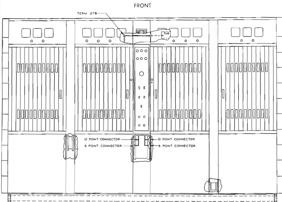
FIG. 2. Lower shows arrangement of cabinets and necessary connections for assembly. Upper shows base diagram of individual units.
