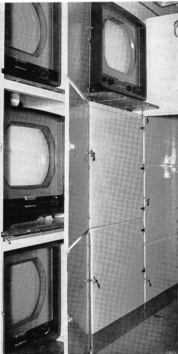
IN THE receiver display unit, shock-mounted compartments provide storage for ten RCA 19-inch TV receivers for transport to various receiving locations. For operation, the receivers are removed, interconnected and placed on special dollies shown on the opposite page. Cables stored in the power unit provide operation of the receivers up to 500 feet from the receiving vehicle.
