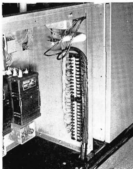
FIG. 11. View showing inter-connecting cables and terminal board "tie" connections.
