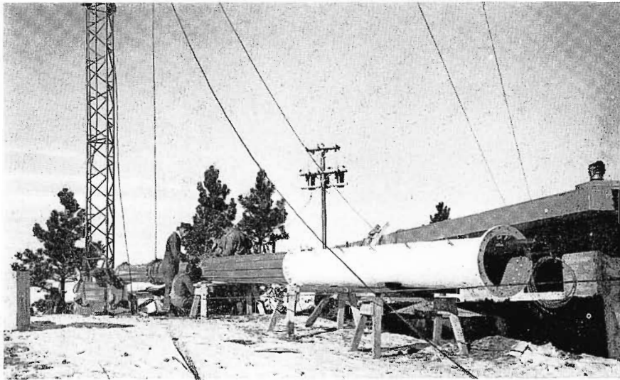
FIG. 9. View of the Pylon FM Antenna during assembly prior to installation.
