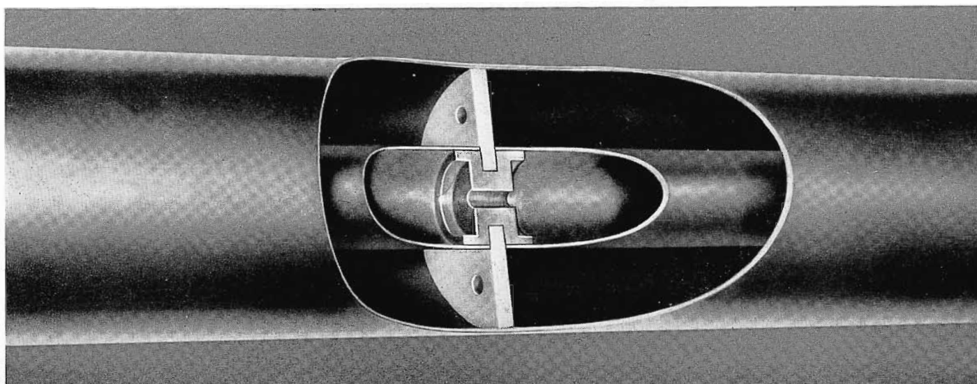
FIG. 1. Photograph of UHF 3 1/8" 50 ohm undercut insulator.
