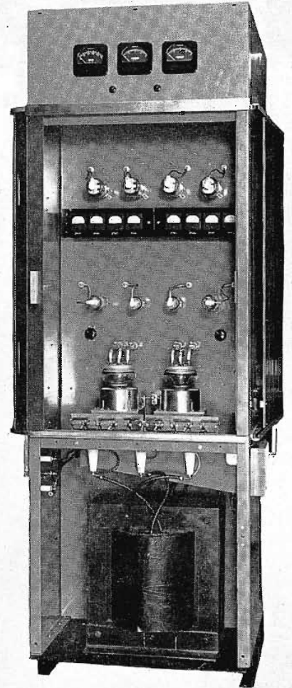
FIG. 19. Front view of modulator which also uses the same type tube, 5762.
