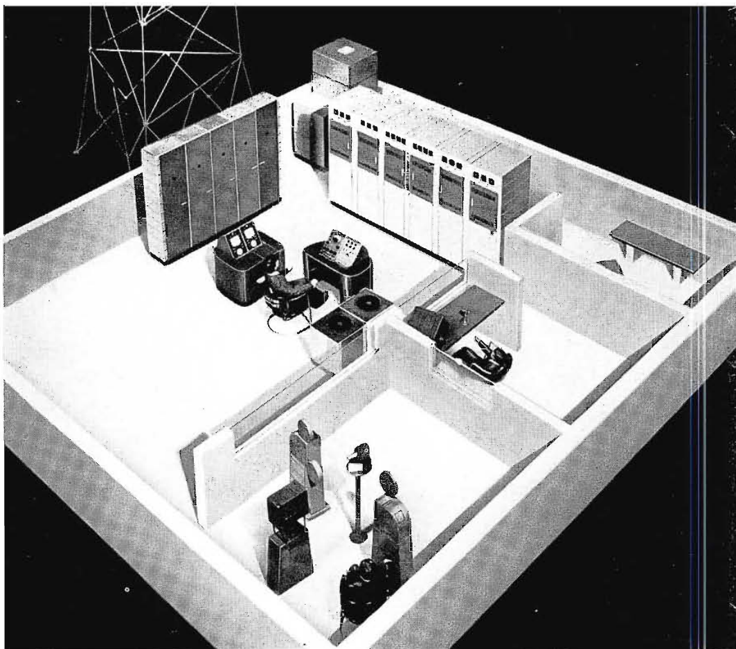
FIG. 4. Model layout of a 10 KW "Basic Buy" station (UHF or VHF). In this set-up, the Console is separated to form a "U" arrangement—with monitors at left and the TC-4A sections in center, and turntables at right.
